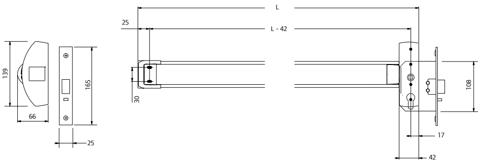
Briton 573 Mortice Nightlatch Operator
