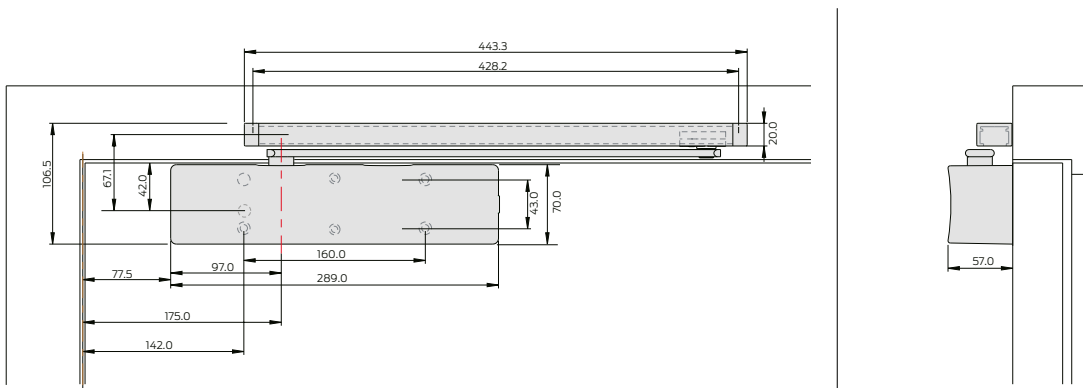
Standard closers with/without mechanical hold open (door mounted - pull side shown).
